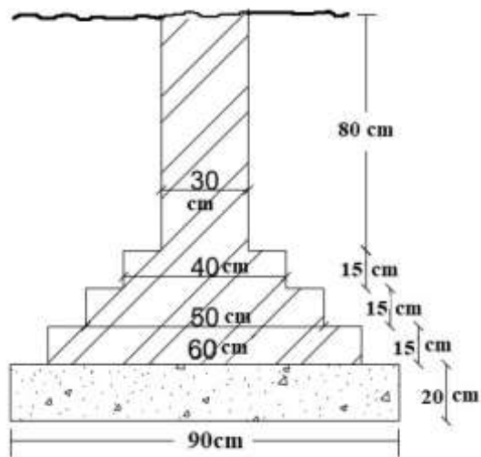
TYPICAL FOUNDATION DETAILS
